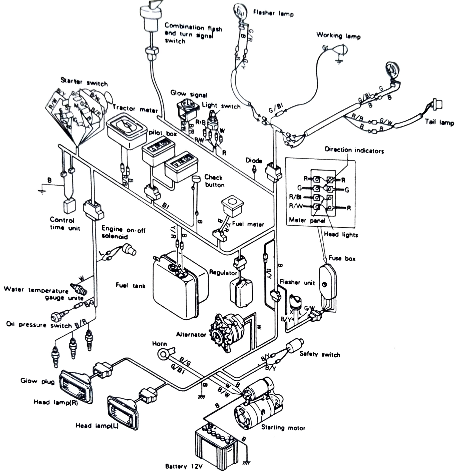
Fig. 75 — Basic electrical diagram for all tractors except Models MT300 and MT300D. Color code is as follows:
